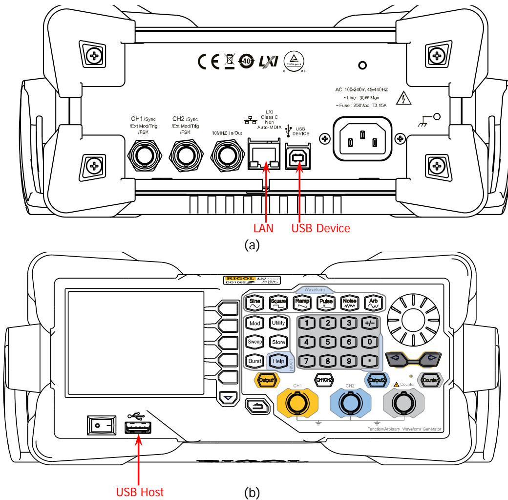
Figure 1-1 DG1000Z Communication Interfaces
