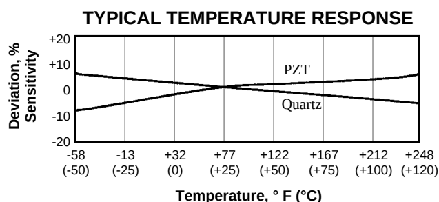
Figure 13. Typical temperature response of PZT and Quartz.
