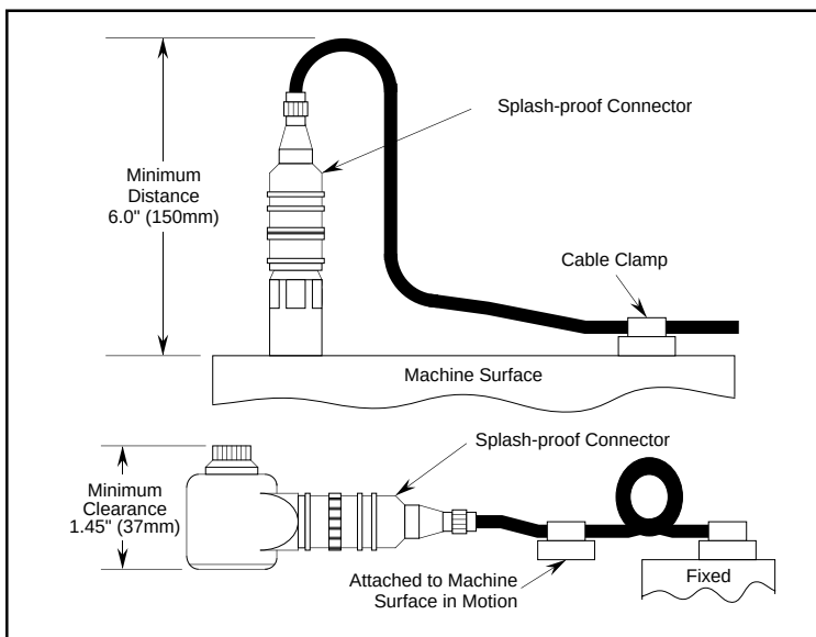
Figure 10. Cable anchoring.
