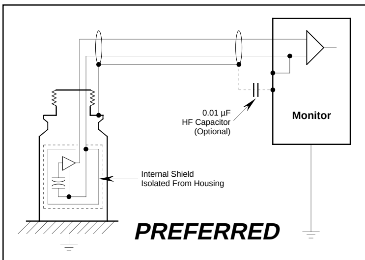
Figure 8. Multiconductor/shield configuration.
