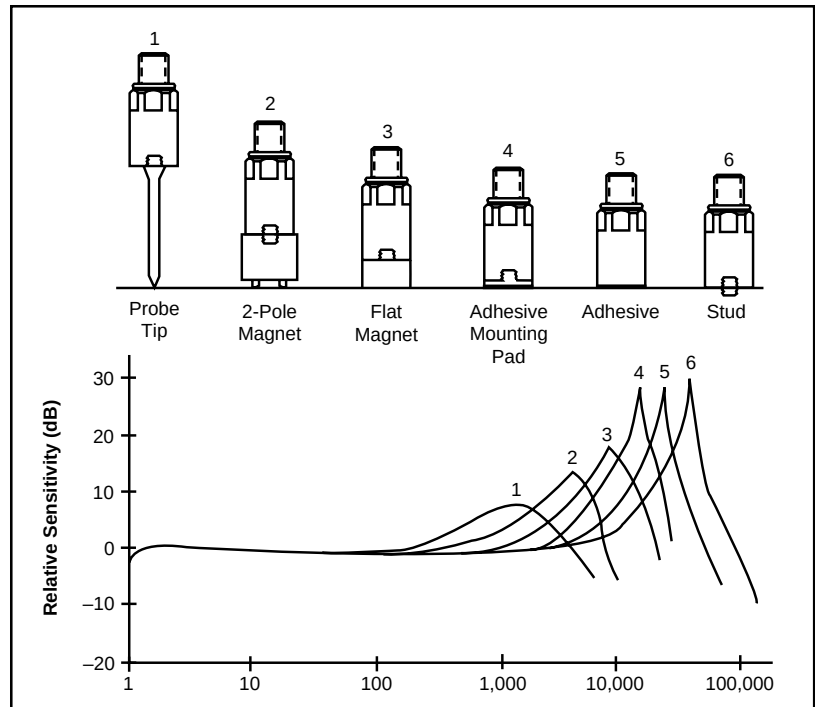
Figure 11. Mounting techniques.
