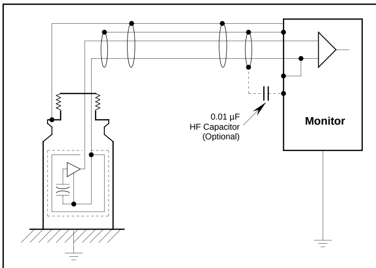
Figure 9. Dual isolated shield configuration.
