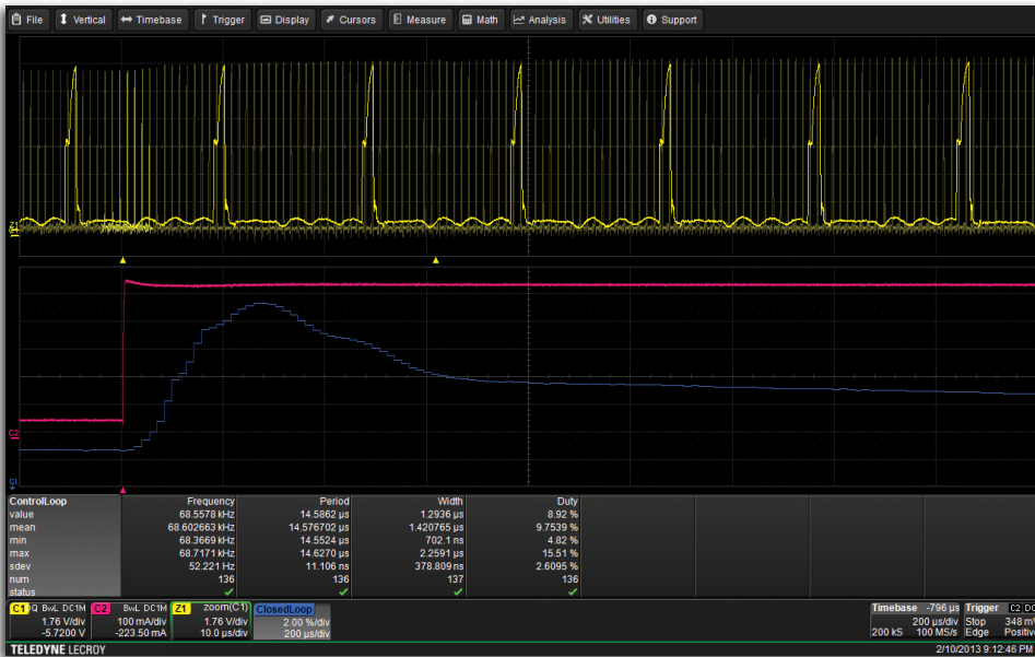
Triggered by the step change in load current (red trace), the gate-drive modulated signal (yellow traces) is captured, the closed-loop, time-domain response of the feedback loop (blue trace) is displayed, confirming loop performance.
