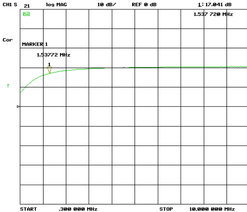
Picture 14 – TBWA2/20dB, gain, 300 kHz – 10 MHz, lin.
