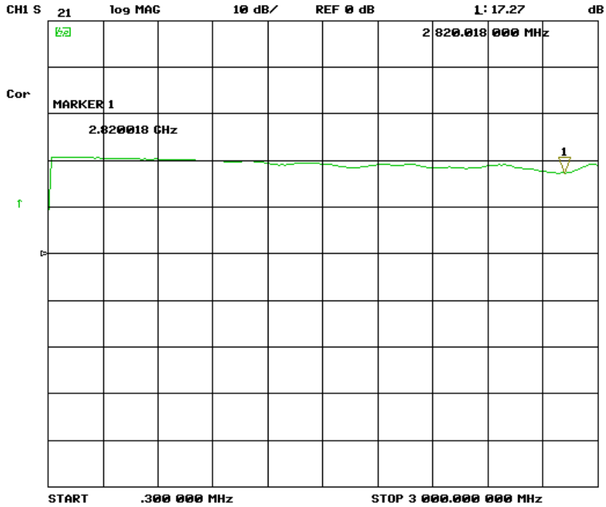
Picture 13 – TBWA2/20dB, gain, 300 kHz – 3 GHz, lin.
