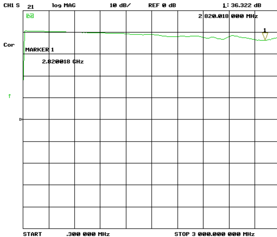
Picture 17 – TBWA2/40dB, gain, 300 kHz – 3 GHz, lin.
