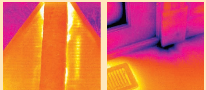
Figure 4. Inspecting to locate air leakage requires a 4 °F or higher temperature difference between inside and outside air, in order to get accurate readings. Air leakage can be into the building, as in the cold air shown leaking through the floor, or out of it, as in the warm air leaking out alongside the chimney. Images courtesy of Snell Infrared ©2005.
