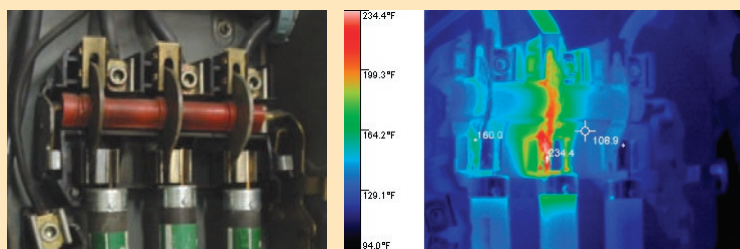
Figure 2. Fused power disconnect and corresponding infrared image.
