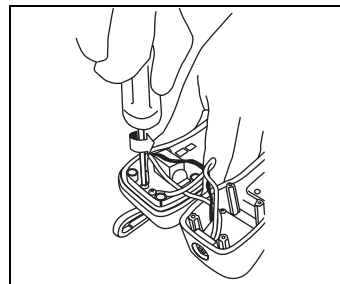
Figure 3. Removing the Line Cord Screws
